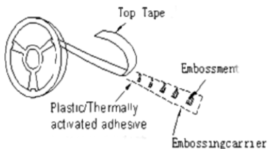
Embossing Tape
